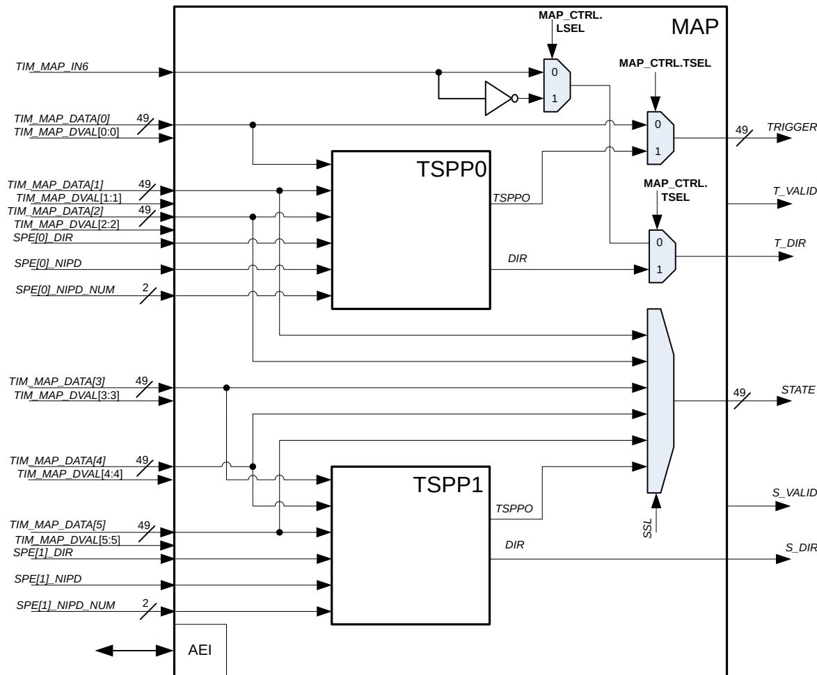
Figure 142 MAP submodule architecture
