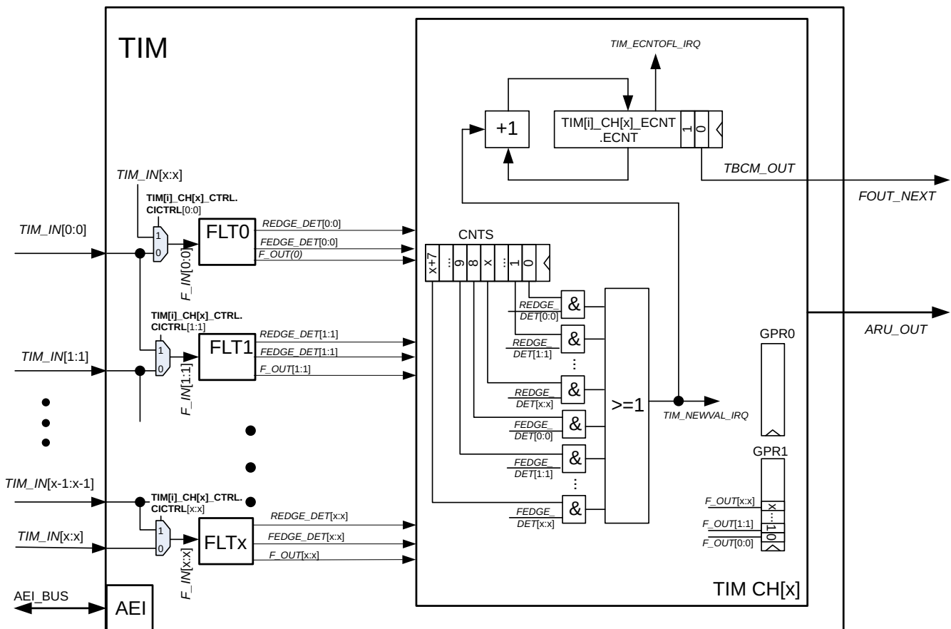
Figure 55 TIM bit compression mode
