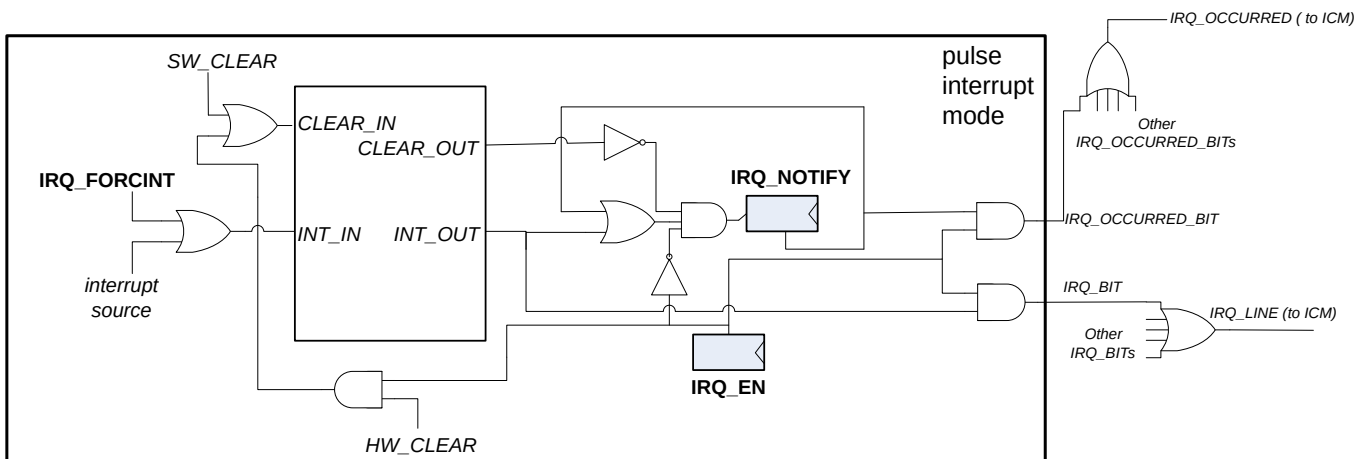
Figure 21 Pulse interrupt mode scheme
