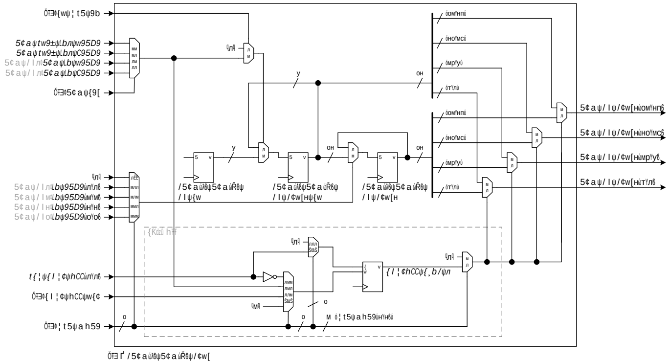
Figure 123 Synchronous update mechanism of register CDTM[i]_DTM[d]_CH_CTRL2
