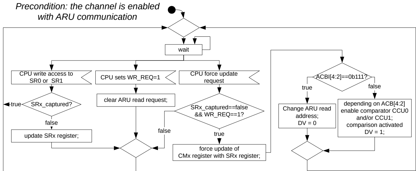
Figure 91 SOMC state diagram for late update requests by configuration interface
