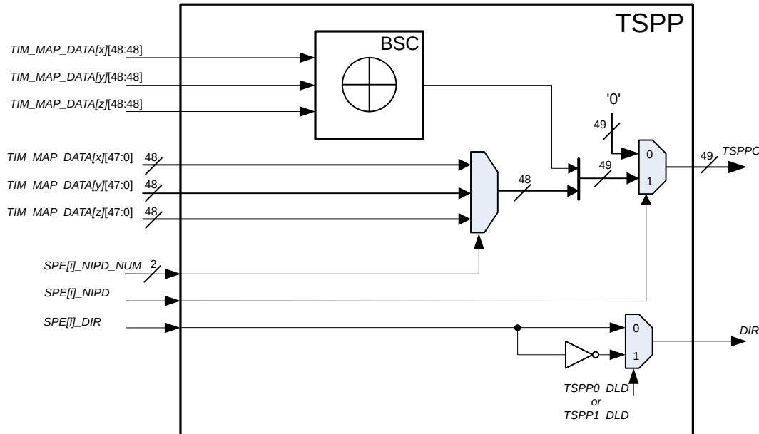
Figure 143 TIM signal preprocessing (TSPP) subunit architecture
