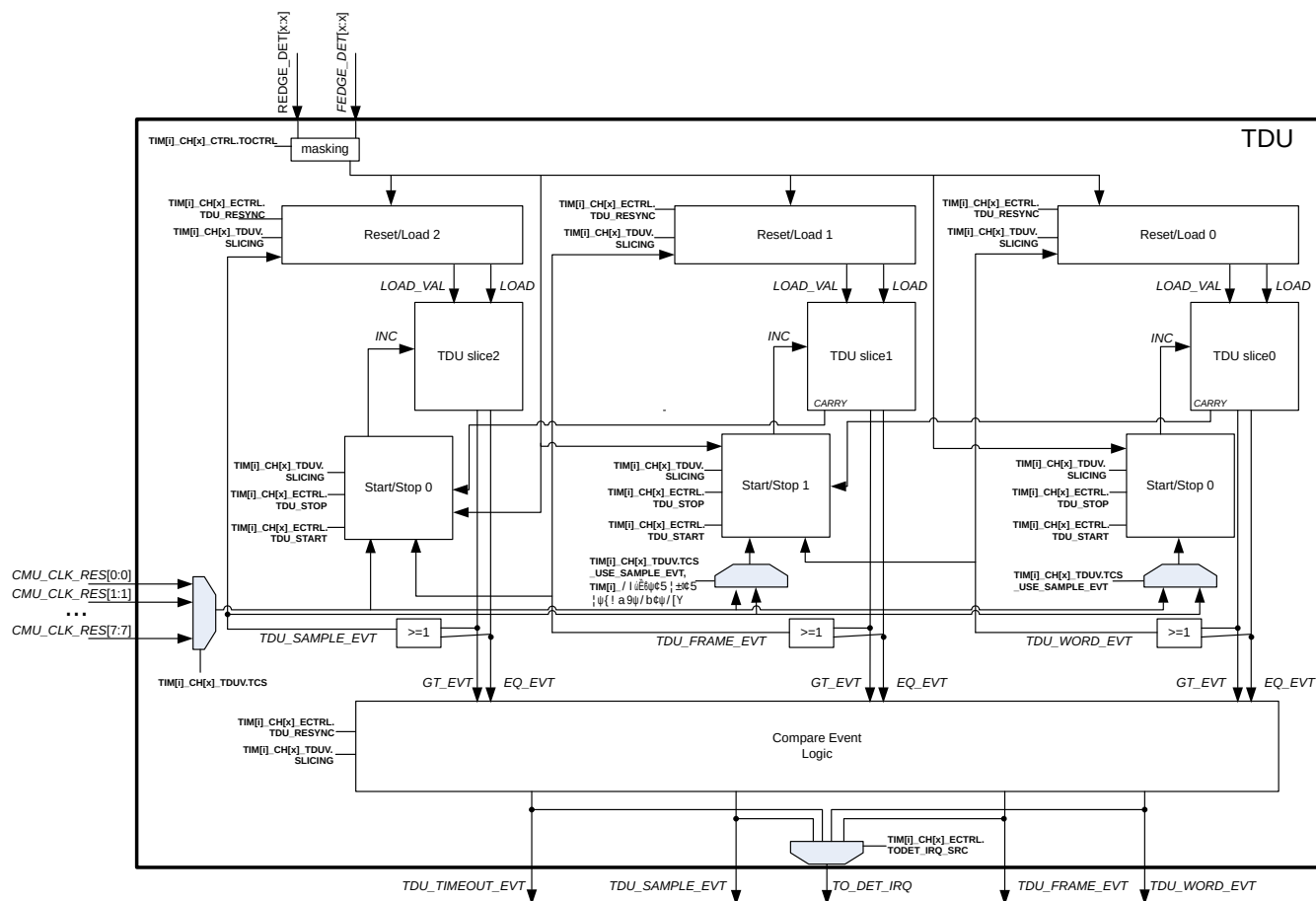
Figure 53 Architecture of the TDU subunit
