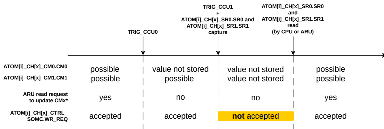
Figure 88 Configuration interface access rights in case of compare strategy 'serve last', ATOM[i]_{CH[x]}_{CTRL\_SOMC}.ABM=1 and ATOM[i]_{CH[x]}_{CTRL\_SOMC}.EUPM=1
