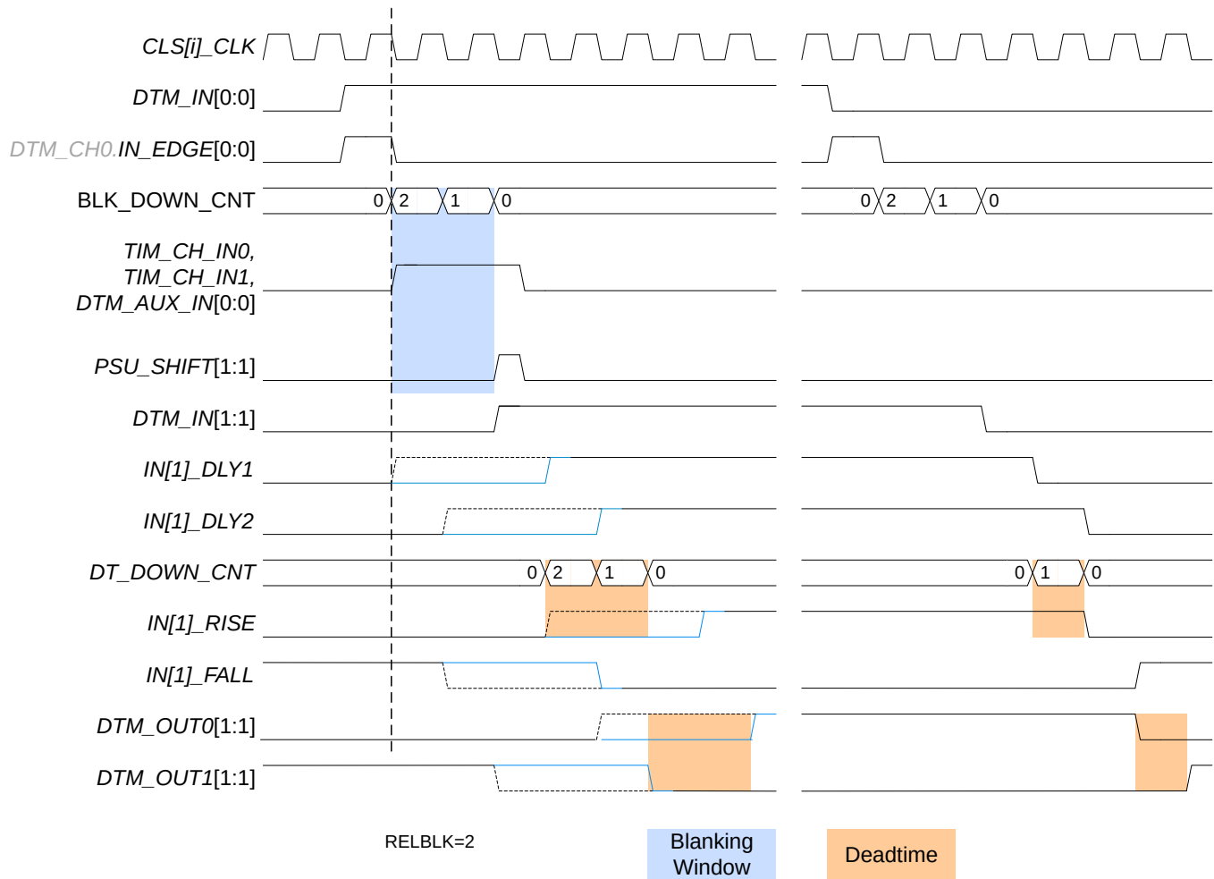
Figure 122 Example wave of phase shift on channel 1
