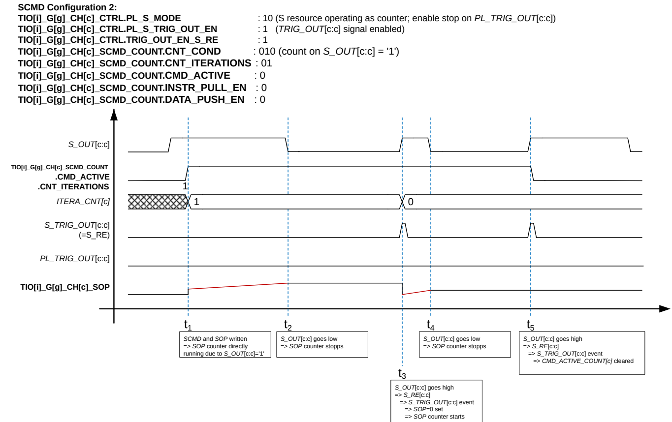
Figure 198 Counting duration of 2 pulses signal S\_OUT[c:c] = 1
