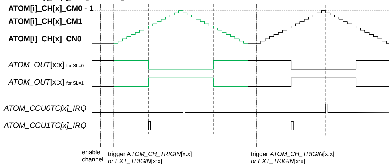
Figure 102 PWM output with respect to configuration bit ATOM[i]_CH[x]_CTRL_SOMP.SL in one-shot counting up-down mode if ATOM[i]_CH[x]_CTRL_SOMP.OSM_TRIG=1
