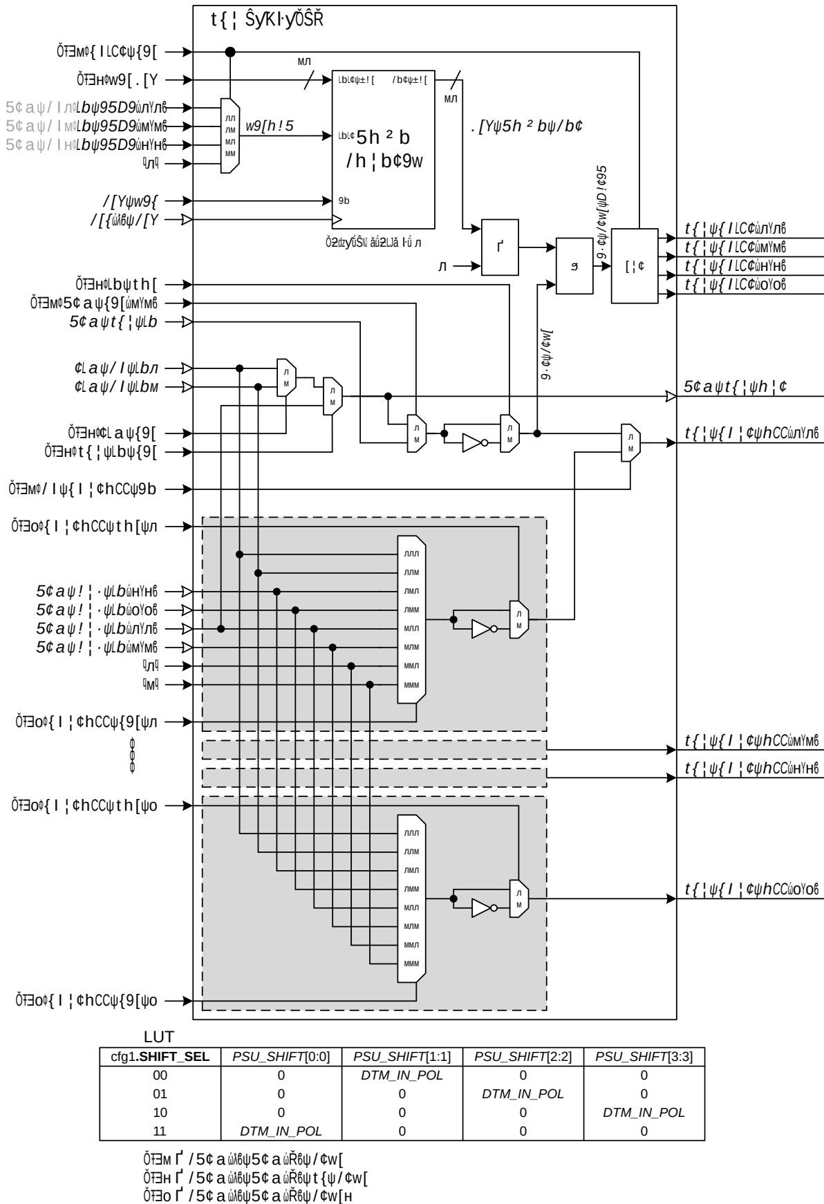
Figure 125 PSU enhanced
