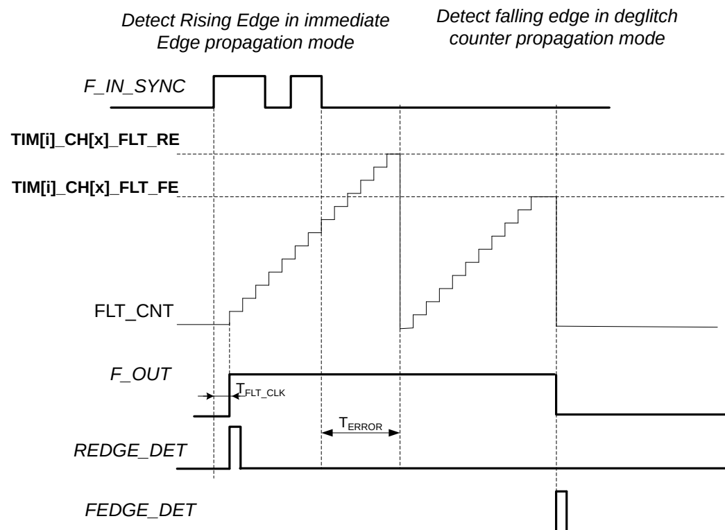
Figure 51 Mixed mode measurement
