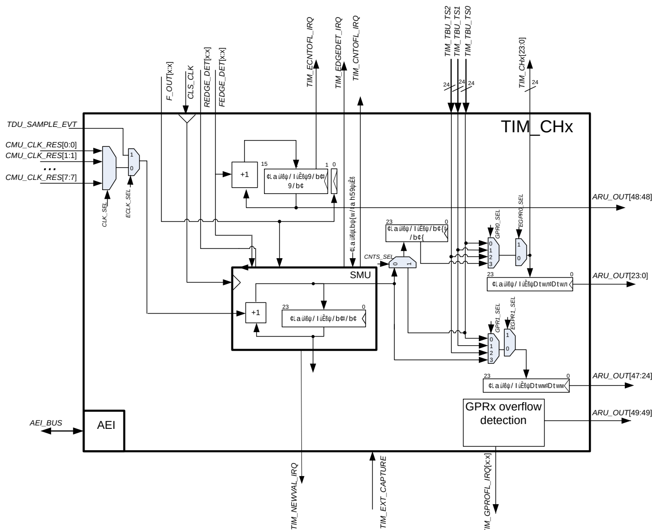
Figure 54 TIM CHx architecture
