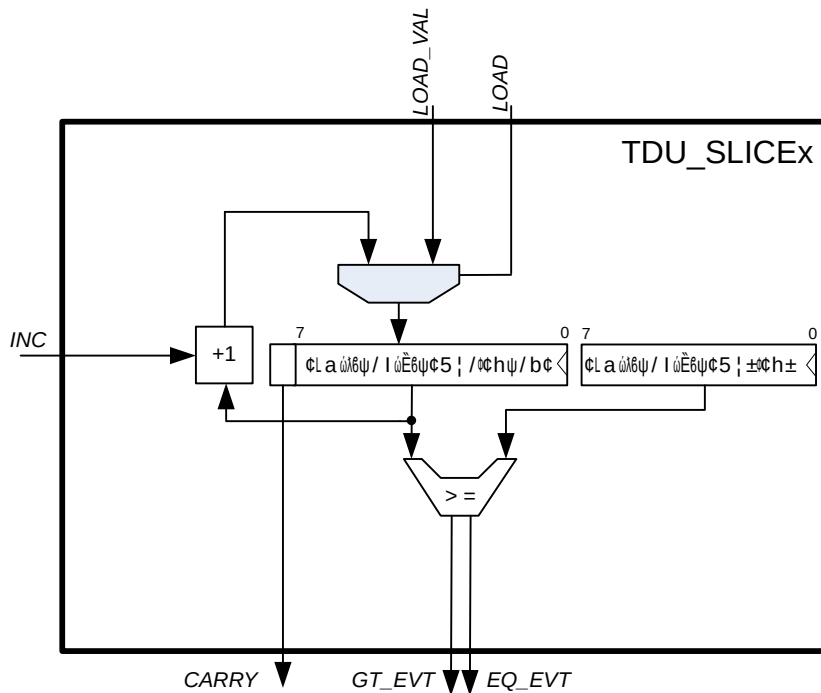
Figure 52 Counter/Comparator slice
