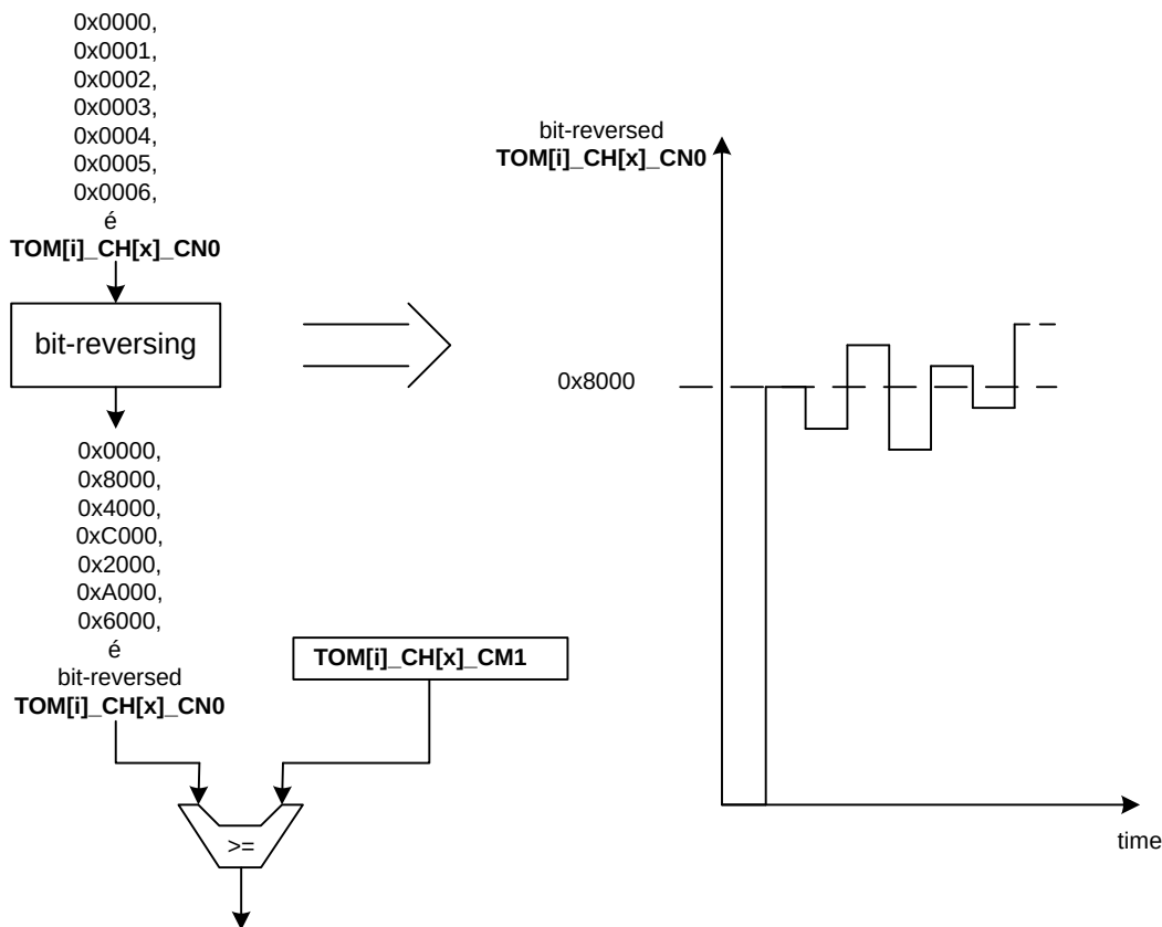
Figure 72 Bit reversing of counter TOM[i]_CH[x]_CN0.CN0 output
