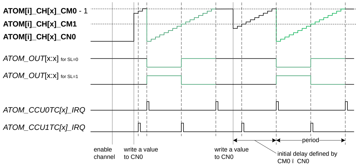
Figure 99 PWM output with respect to configuration bit ATOM[i\_CH[x]]\_CTRL\_SOMP.SL in one-shot counting up mode if ATOM[i\_CH[x]]\_CTRL\_SOMP.OSM\_TRIG=0
