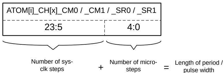
Figure 105 Period and duty cycle register in HRES mode
