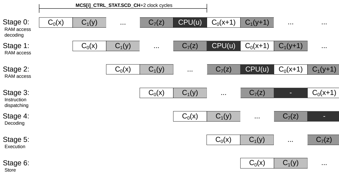
Figure 134 Timing of round-robin scheduling
