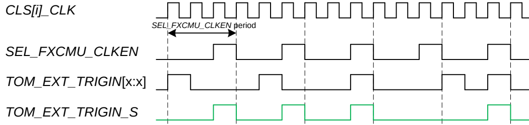
Figure 61 Timing diagram of RS unit
