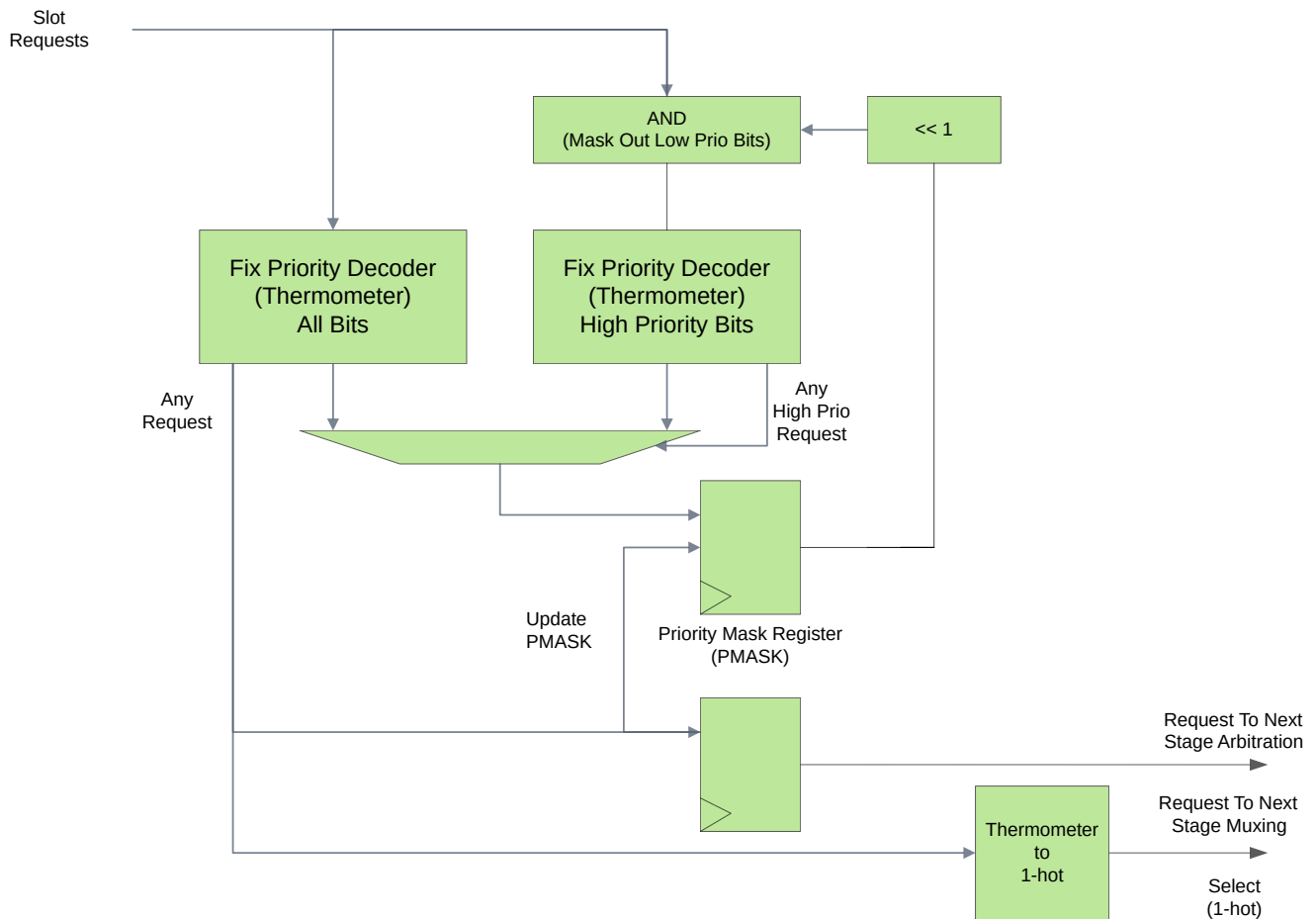
Figure 32 Round-robin arbiter
