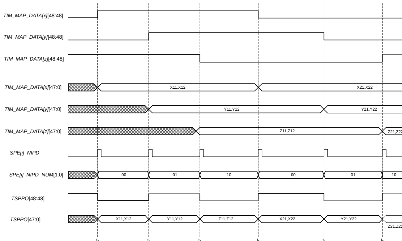
Figure 144 TSPP signal generation for signal TSPPO
