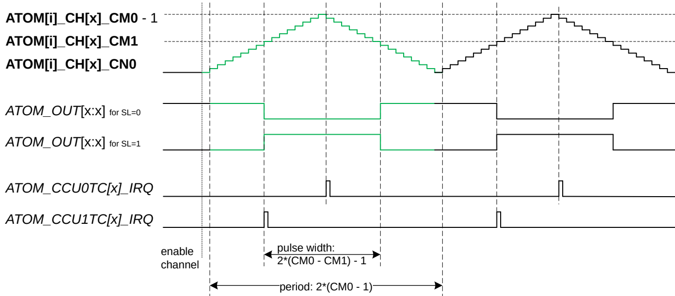
Figure 97 PWM output behavior with respect to the ATOM[i]_CH[x]_CTRL_SOMP.SL bit in continuous counting up-down mode if ATOM[i]_CH[x]_CTRL_SOMP.RST_CCU0=0
