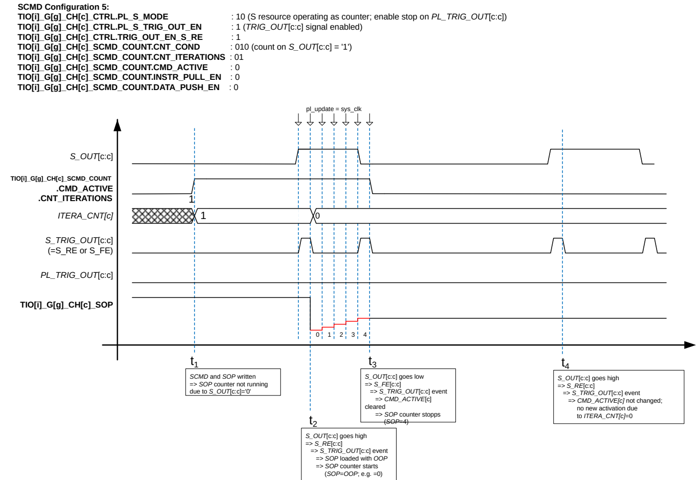
Figure 197 Counting duration of 1 high pulse signal S_OUT[c:c]
