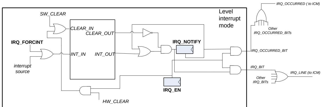
Figure 19 Level interrupt mode scheme
