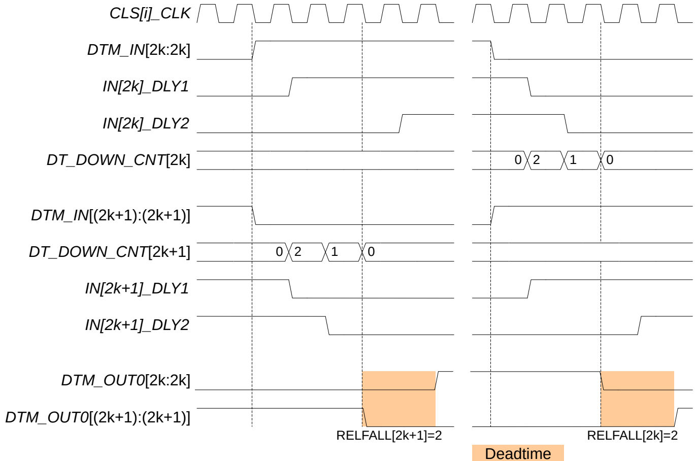
Figure 119 Cross channel dead time timing diagram
