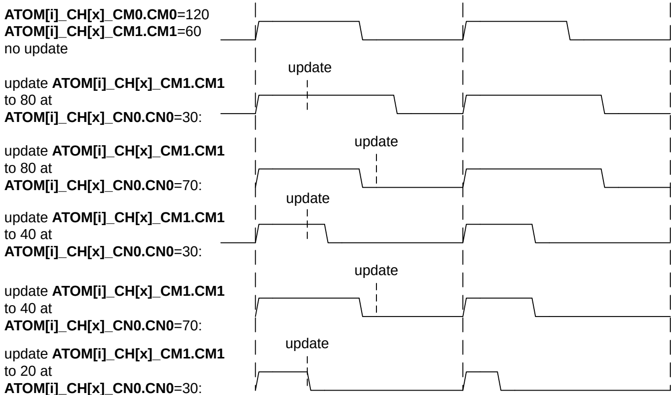
Figure 93 Asynchronous update of pulse width only in SOMP continuous counting up mode with \text{ATOM}[i]_{\text{CH}[x]}_{\text{CTRL.RST\_CCU0}}=0
