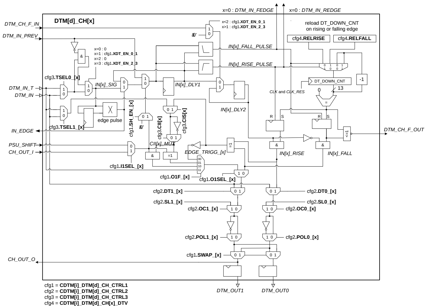
Figure 117 DTM channel overview
