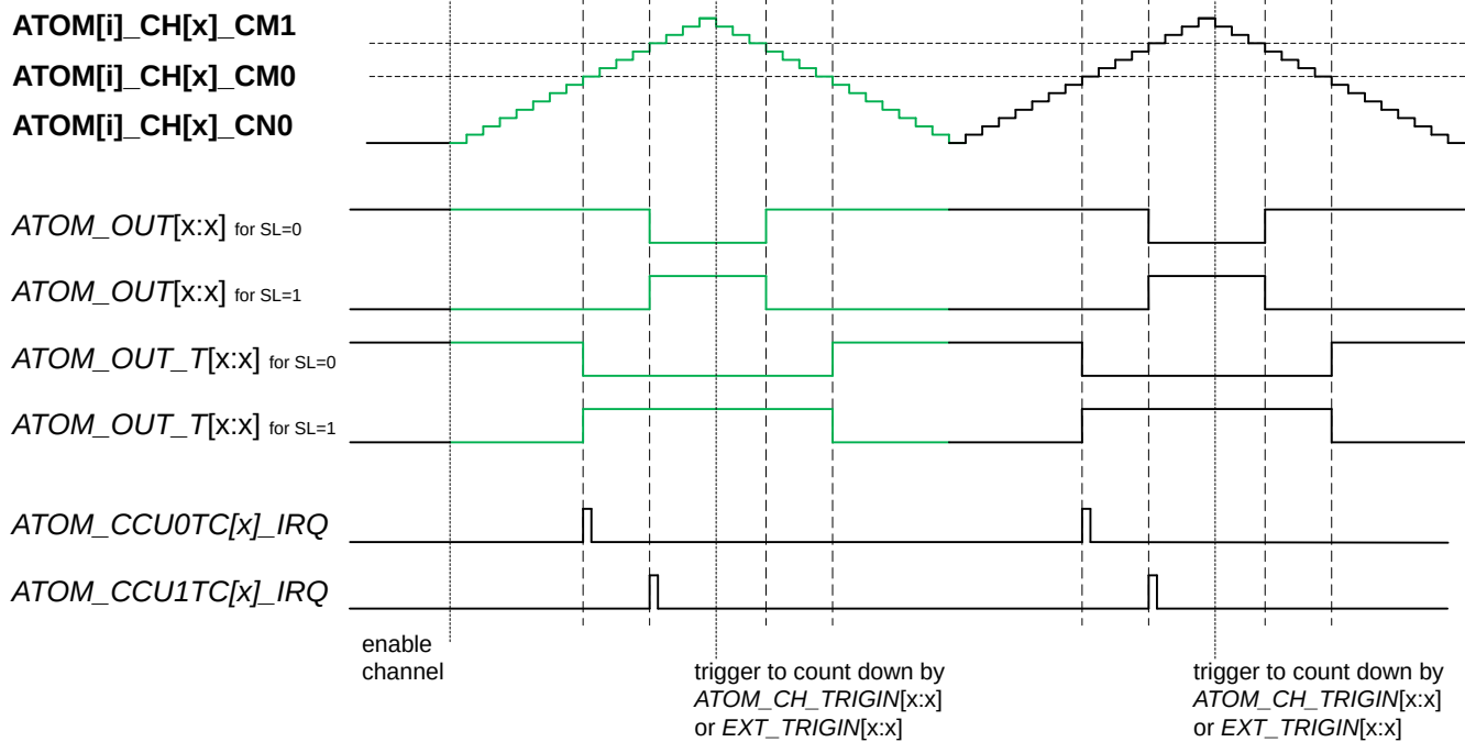
Figure 98 PWM output behavior with respect to the ATOM[i]_CH[x]_CTRL_SOMP.SL bit in continuous counting up-down mode if ATOM[i]_CH[x]_CTRL_SOMP.RST_CCU0=1
