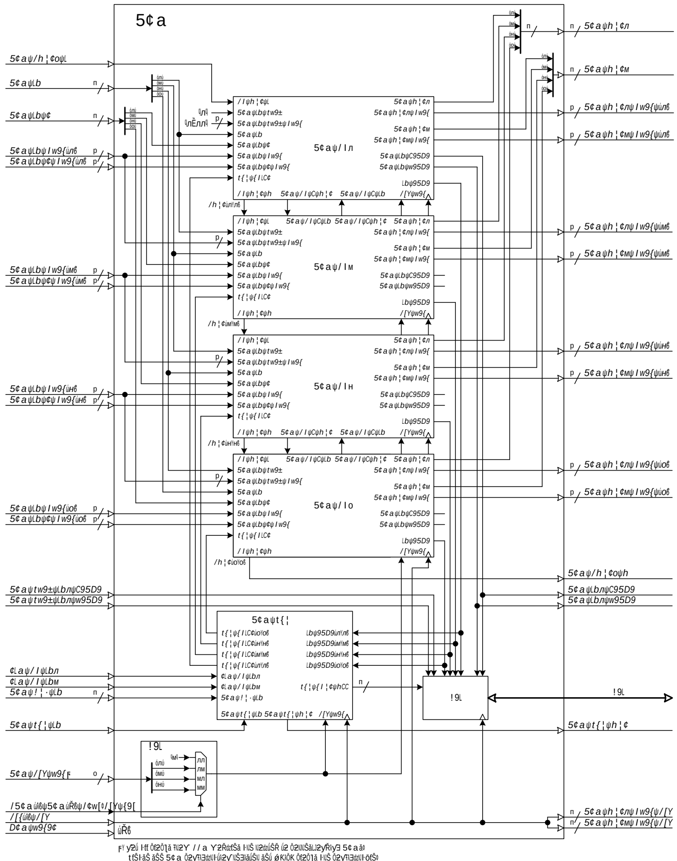
Figure 115 DTM overview
