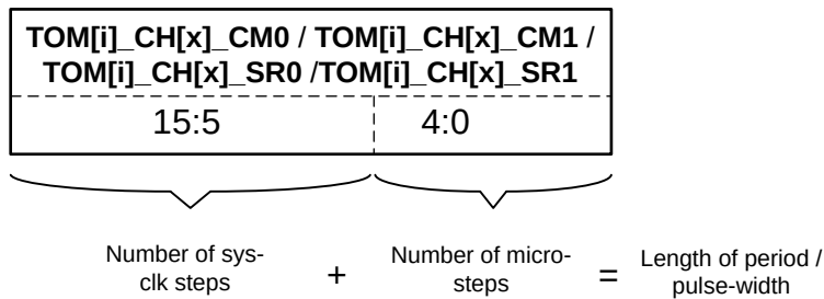
Figure 74 Period and duty cycle register in HRES mode
