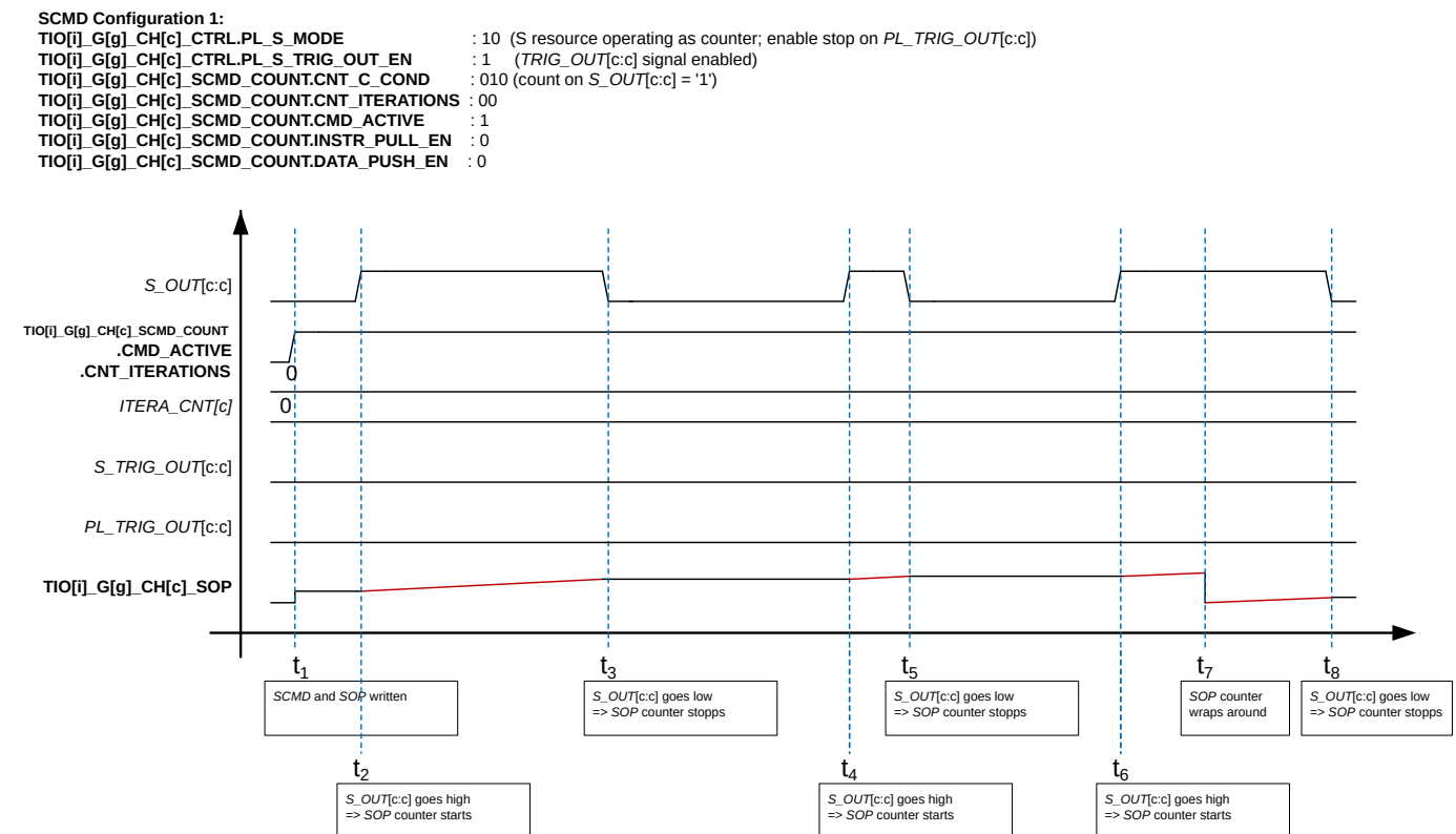
Figure 196 Endless counting signal S_OUT[c:c] = 1
