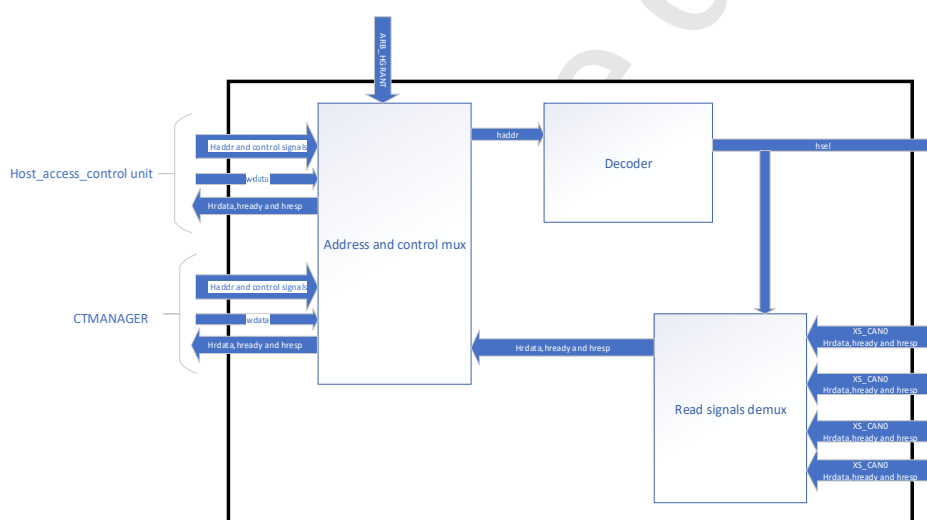
Figure 5. AHB Control Multiplexer and Decoder Block Diagram
