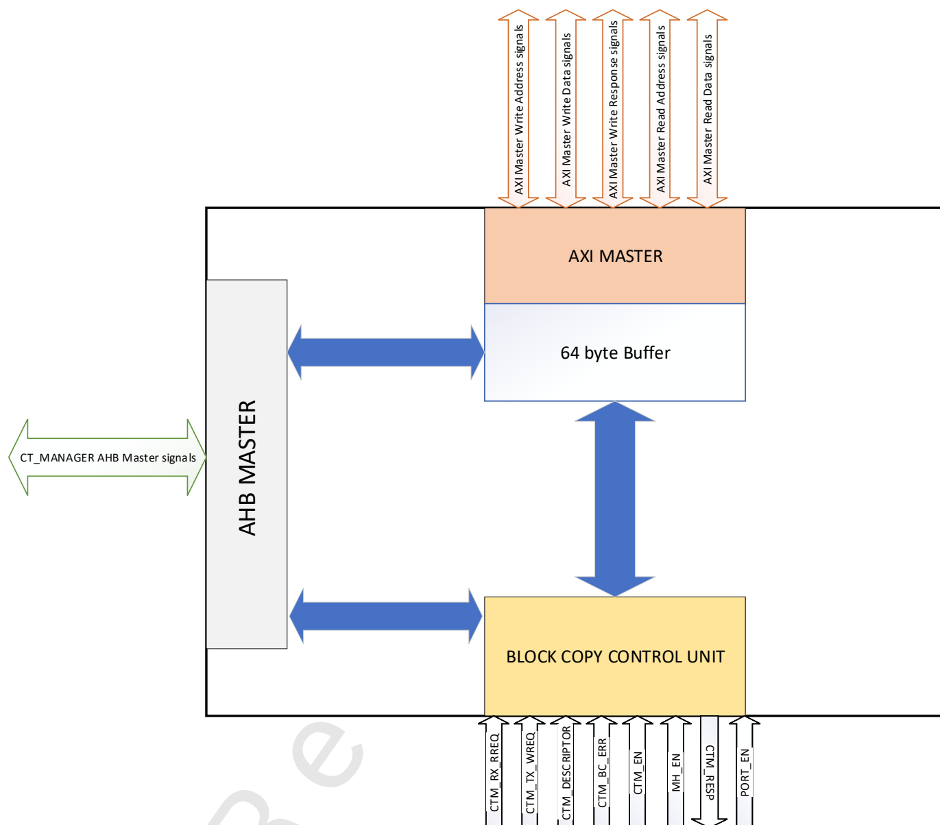
Figure 2. CT_MANAGER Block Diagram
