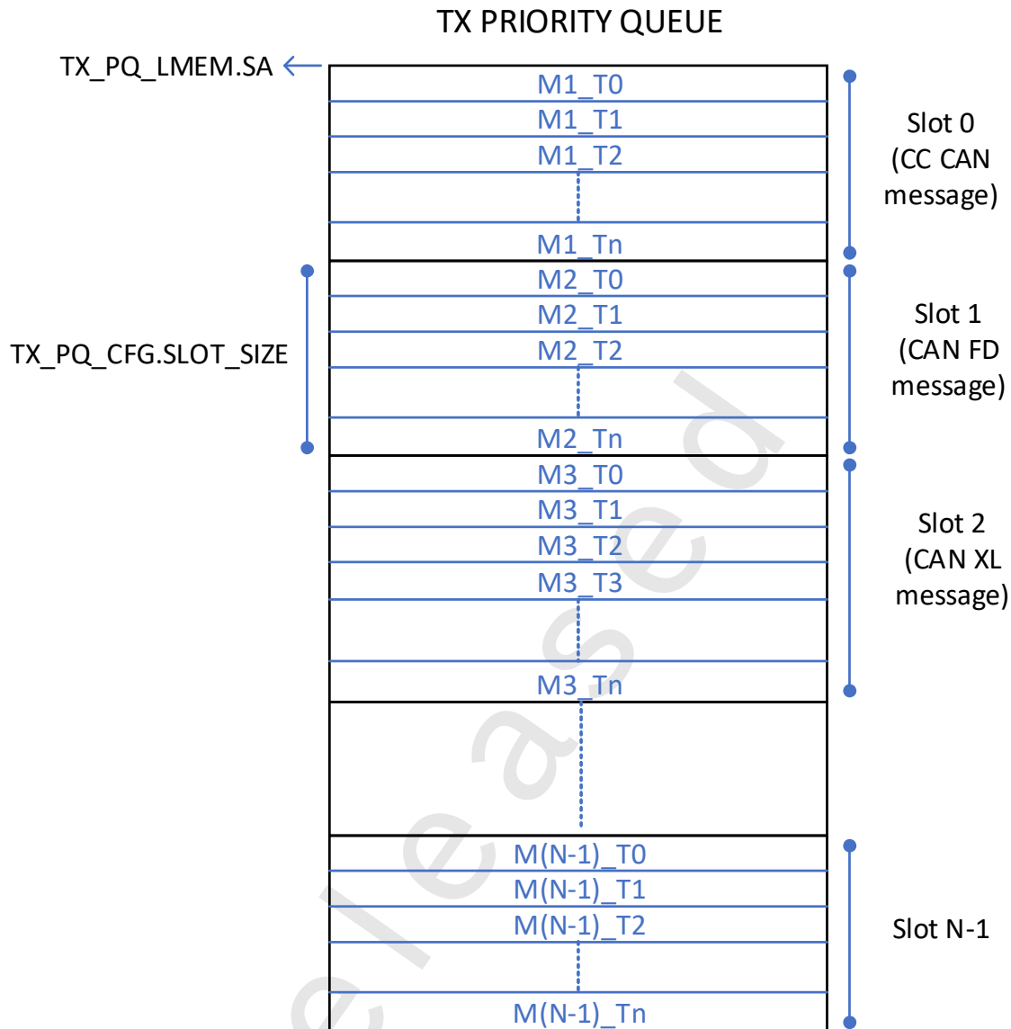
Figure 6. TX Priority Queue Configuration
