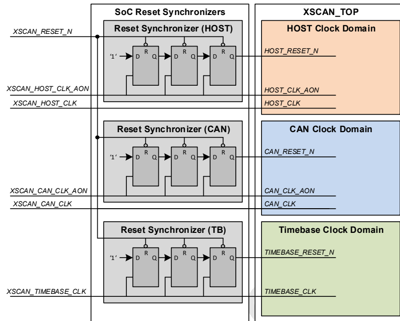
Figure 80. XS_CAN_TOP Reset Circuit
