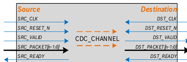
Figure 68. CDC_CHANNEL
