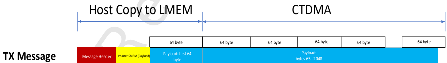
Figure 21. TX in CTM
