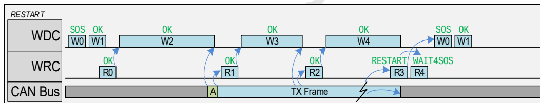
Figure 40. TX_MSG Sequence with Code RESTART
