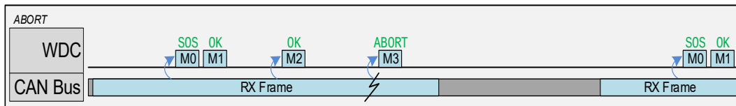
Figure 49. RX_MSG Sequence with Code ABORT
