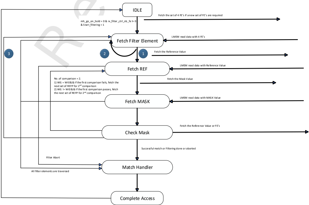
Figure 19. RX Filtering
