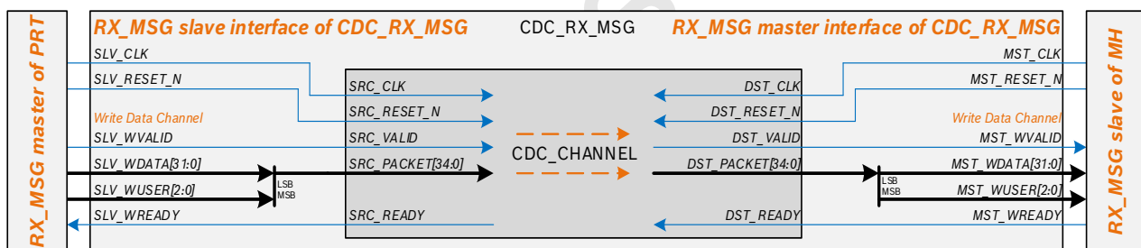
Figure 71. CDC_RX_MSG
