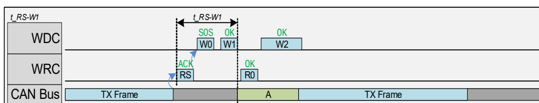
Figure 44. TX_MSG Sequence Timing t_{RS-W1}
