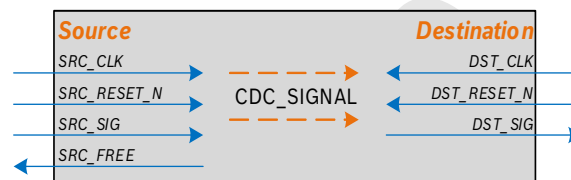
Figure 62. CDC_SIGNAL
